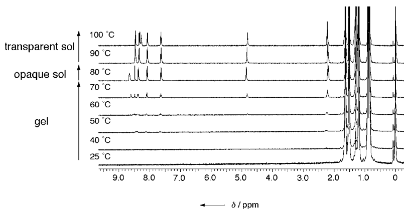
Figure 6. : Variable temperature 400 MHz ^1\text{H} NMR spectra of compound 1 (10.0mm) in [\text{D}_{18}] decaline.
