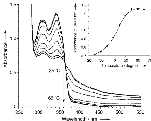
Figure 4. Temperature dependent UV-visible spectra of compound 1 (0.10 mM) in decaline (inset: absorbance at 349.0 nm at different temperatures).
