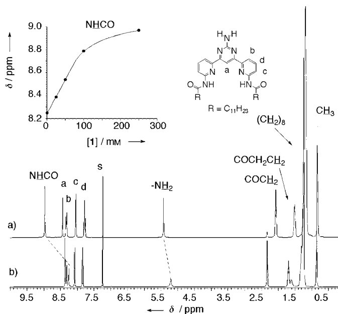
Figure 1. 400 MHz 1 H NMR spectra of 1 in [D 1 ]CHCl 3 a) 250.0 mM, b) 1.0 mM (s: solvent, inset: concentration dependence of chemical shift of the amide protons) at 25 °C.
