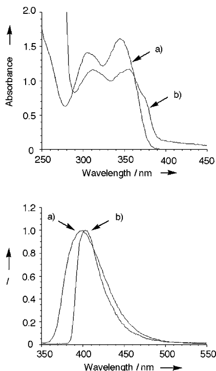
Figure 3. UV-visible spectra (top) and fluorescence spectra (bottom) ( \lambda_{\text{ex}} = 340.0 nm) of 1 (0.10 mM) in a) chloroform and b) decaline at 25 °C.
