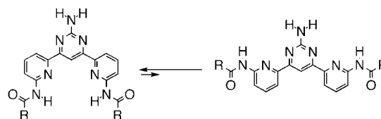
Scheme 2. Preferred conformation of compound 1 .
