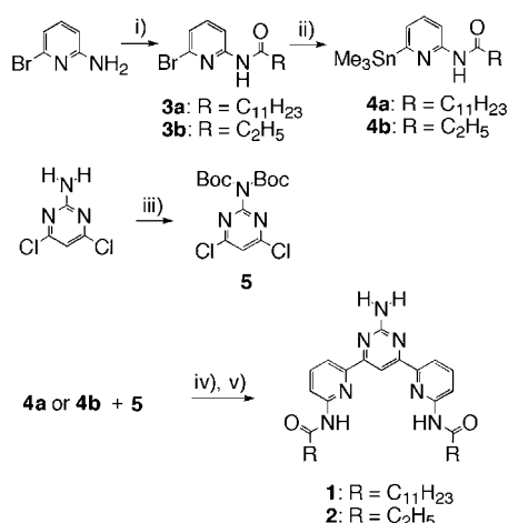
Scheme 3. i) RCOCl, Py, CH 2 Cl 2 , room temperature; ii) Me 3 SnSnMe 3 , 5 mol % [Pd(PPh 3 ) 4 ], PhMe, 110 °C; iii) (Boc) 2 O, DMAP, CH 2 Cl 2 , room temperature; iv) 5 mol % [Pd(PPh 3 ) 4 ], DMF, 110 °C; v) TFA, CH 2 Cl 2 , room temperature.
