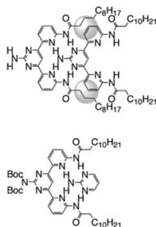
Figure 2. Schematic representation of the shielding effect due to the pyridine rings.
