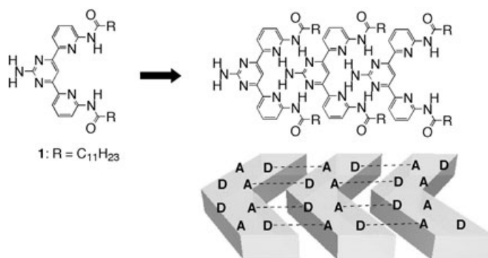
Scheme 1. Structure of the monomer 1 bearing self-complementary DAAD–ADDA patterns of hydrogen bonding sites and its directional self-assembly into a ribbon-like supramolecular polymer through an array of four hydrogen bonds.
