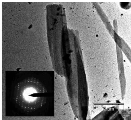
Figure 5. Electron micrograph of compound 1 in decaline (1.0mm) obtained by the direct observation technique, (inset: selected area electron diffraction pattern).
